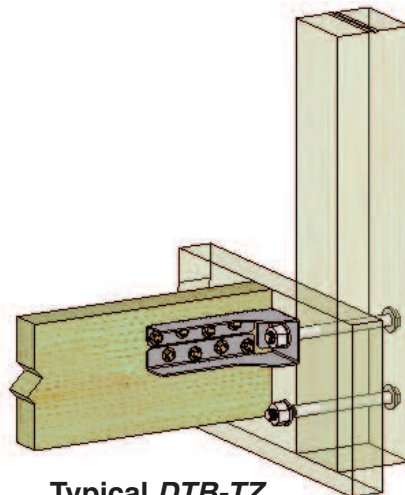
Typical DTB-TZ installation
