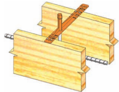
Typical ABHS12 installation
