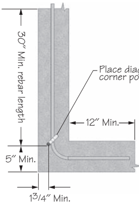
Plan View of Corner installation
