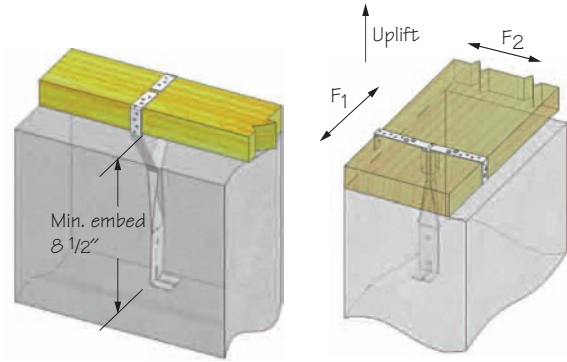
Typical ST1-TZ installation in concrete
