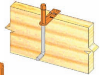
Typical ABH12 installation
