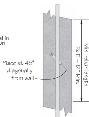
Plan View of Continuous stem wall installation
