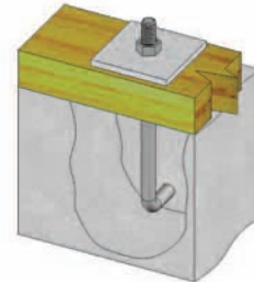
Typical AB128 installation
