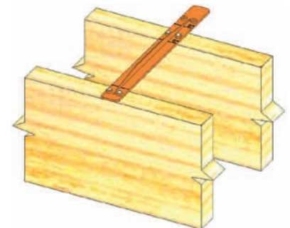
Typical FBS installation
