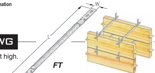
Typical FT/WG installation
