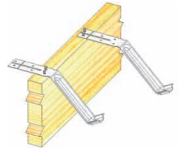
FA3 Form board installation
