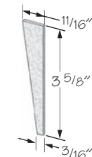
WG Wedge must order separately
