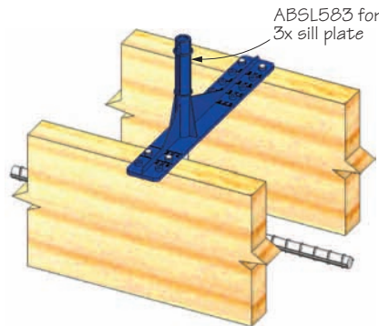
Typical ABHS58 installation
