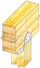
Typical C44 installation
