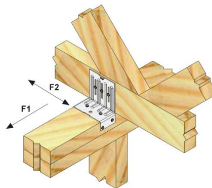
TYPICAL HTC4 INSTALLATION
