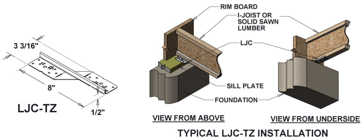
FIGURE 6 – LJC-TZ LATERAL JOIST CONNECTOR
