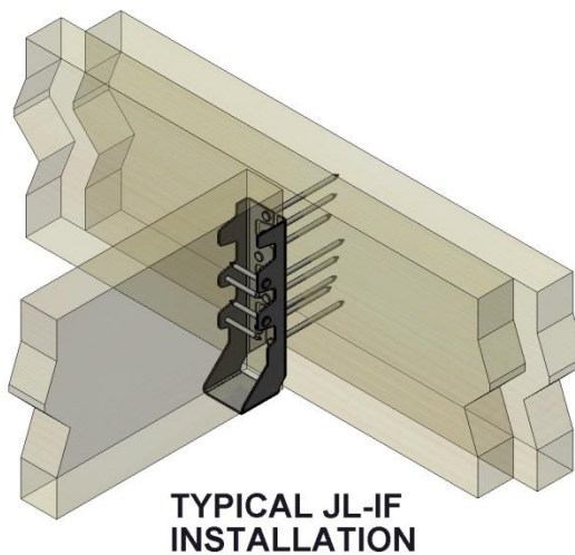
FIGURE 5 – JLIF-TZ INVERTED FLANGE JOIST HANGERS
