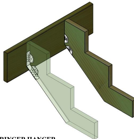
FIGURE 1 – CSH-TZ CONCEALED STRINGER HANGER
