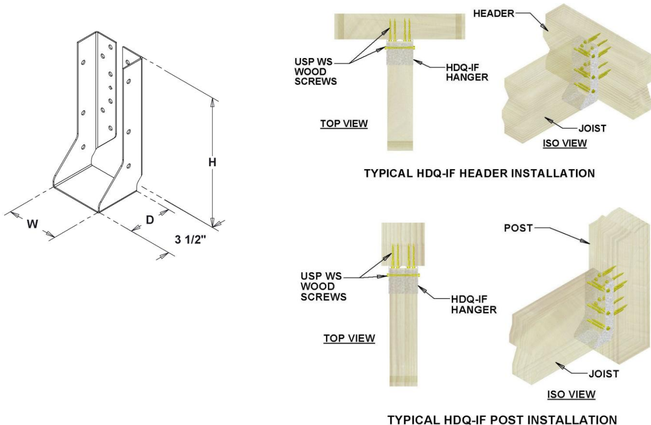
FIGURE 2 – HDQIF FACE MOUNT INVERTED FLANGE HANGERS
