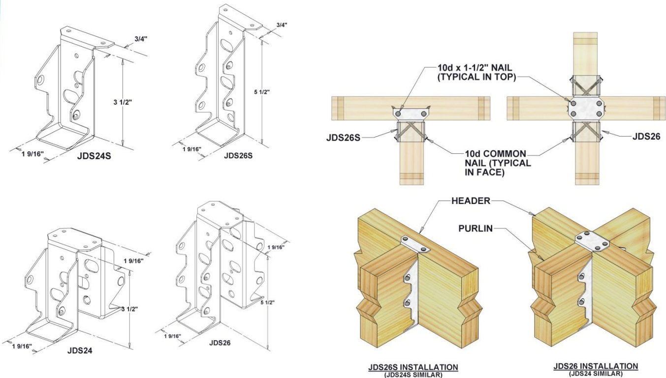
TYPICAL JDS PURLIN HANGER INSTALLATION
