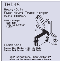
Installation Detail
