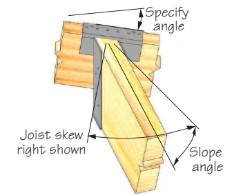
Specify angle Joist skew right shown Slope angle Typical HLBH hanger skewed right, sloped down, top flange sloped
