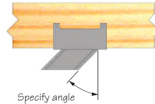
Specify angle Typical PHXU hanger skewed, left shown Type A (bevel cut required)
