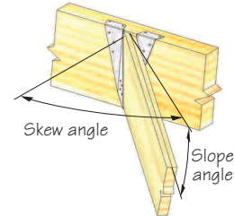
Typical BPH hanger sloped down, skewed right, low side flush shown
