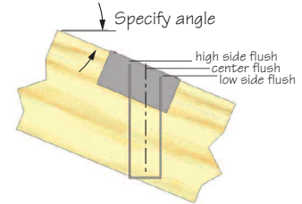
Typical HLBH hanger sloped top flange right shown
