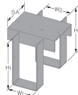
Typical PHXU hanger saddle option
