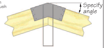
Specify angle Typical HLBH hanger ridge, top flange slope
