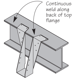
Typical Top Flange welded installation
