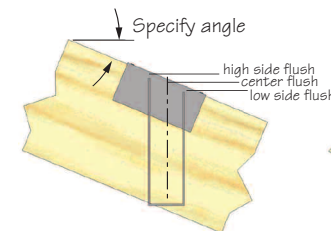
Specify angle Typical HLBH hanger sloped top flange, right shown
