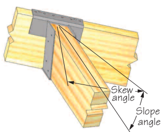
Typical HLBH hanger sloped down, skewed right, low side flush shown
