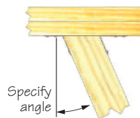
Typical SUH hanger skewed, right shown, Type A (bevel cut required)
