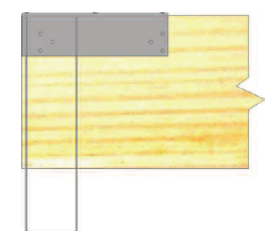
Typical HLBH hanger top flange offset, right shown
