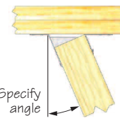
Typical SUH formed hanger skewed, right shown, Type B
